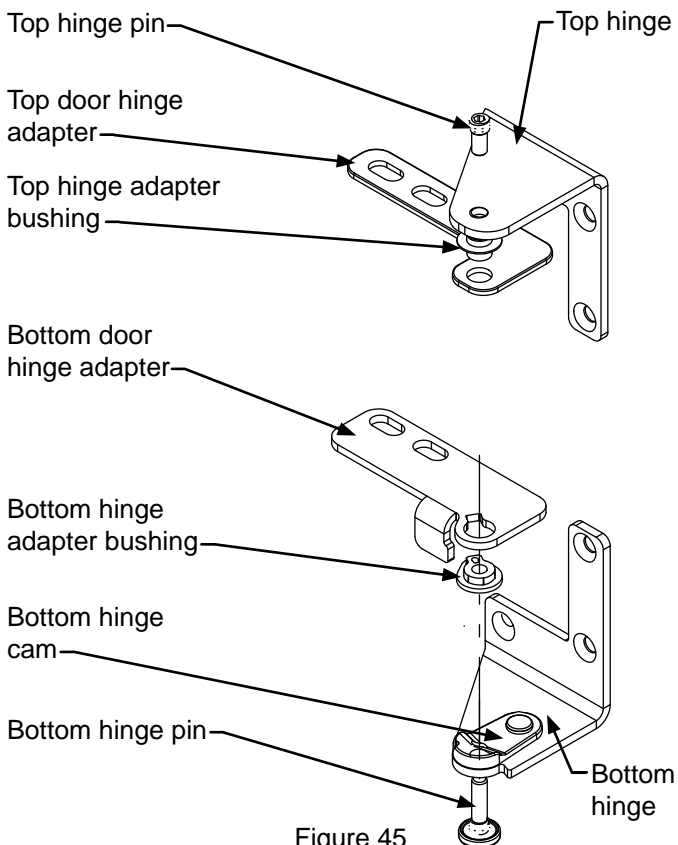
Figure 45 Right hand hinges shown
