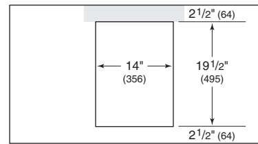
COUNTERTOP CUT-OUT
